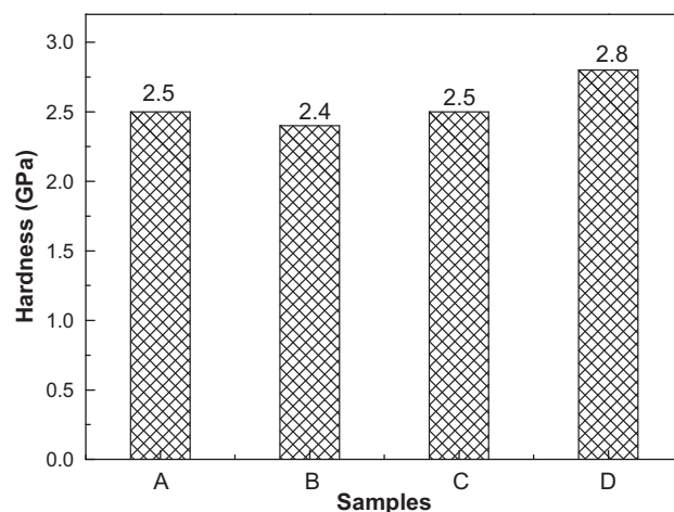
Fig. 6. Vickers hardness of A, B, C and D alloys.
